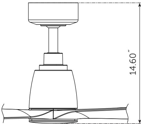
6" downrod
