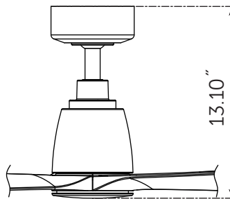
4.5" downrod
