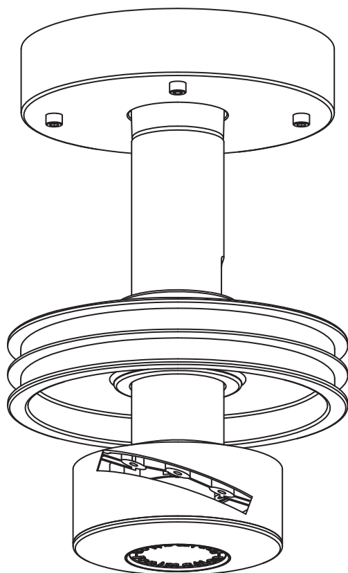
Pulley Assembly (1)
